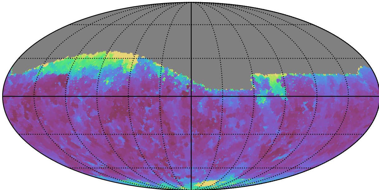
ddf_loaded_half_fl8_v3.4_10yrs Yr 1 r band: Min seeingGeom
