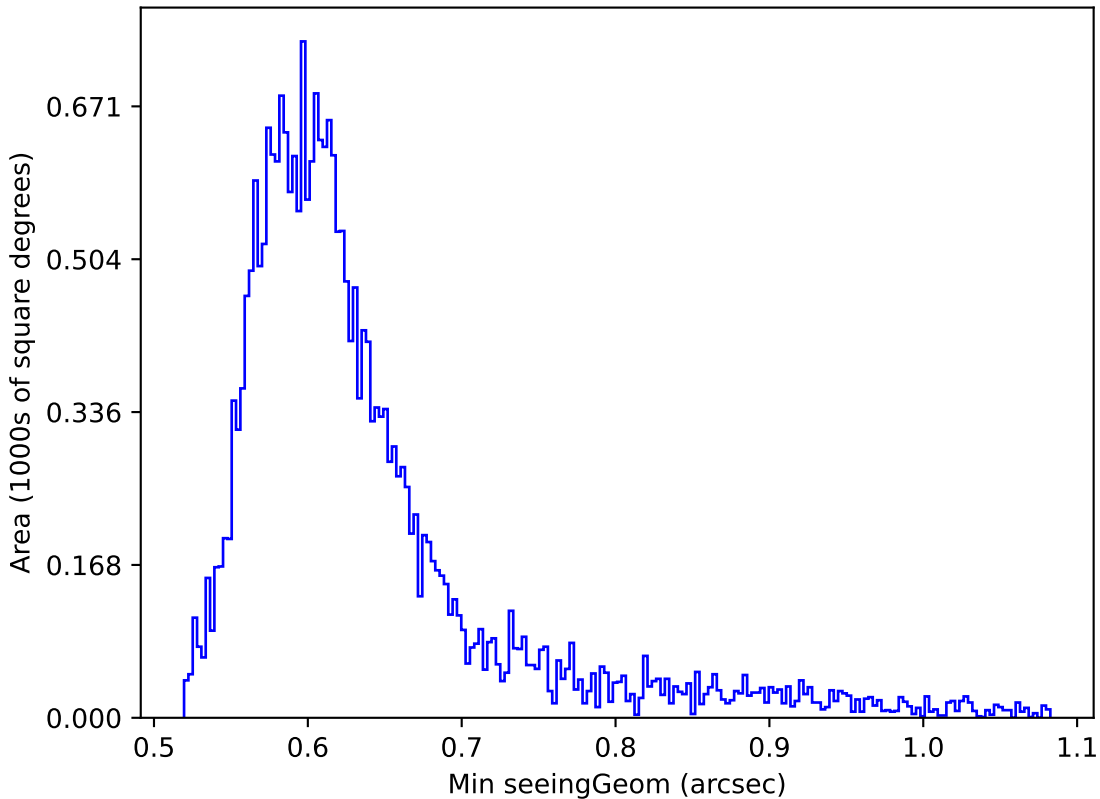
ddf_loaded_half_fl8_v3.4_10yrs Yr 1 r band: Min seeingGeom
