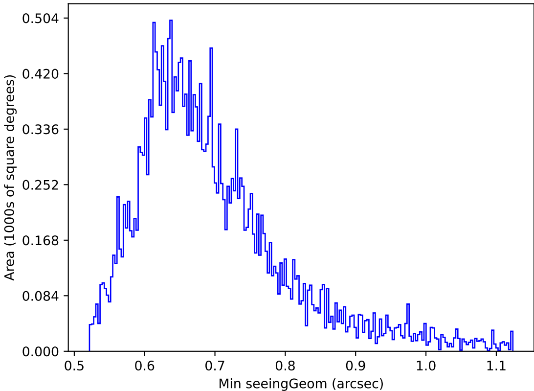
ddf_loaded_half_fl8_v3.4_10yrs Yr 1 g band: Min seeingGeom
