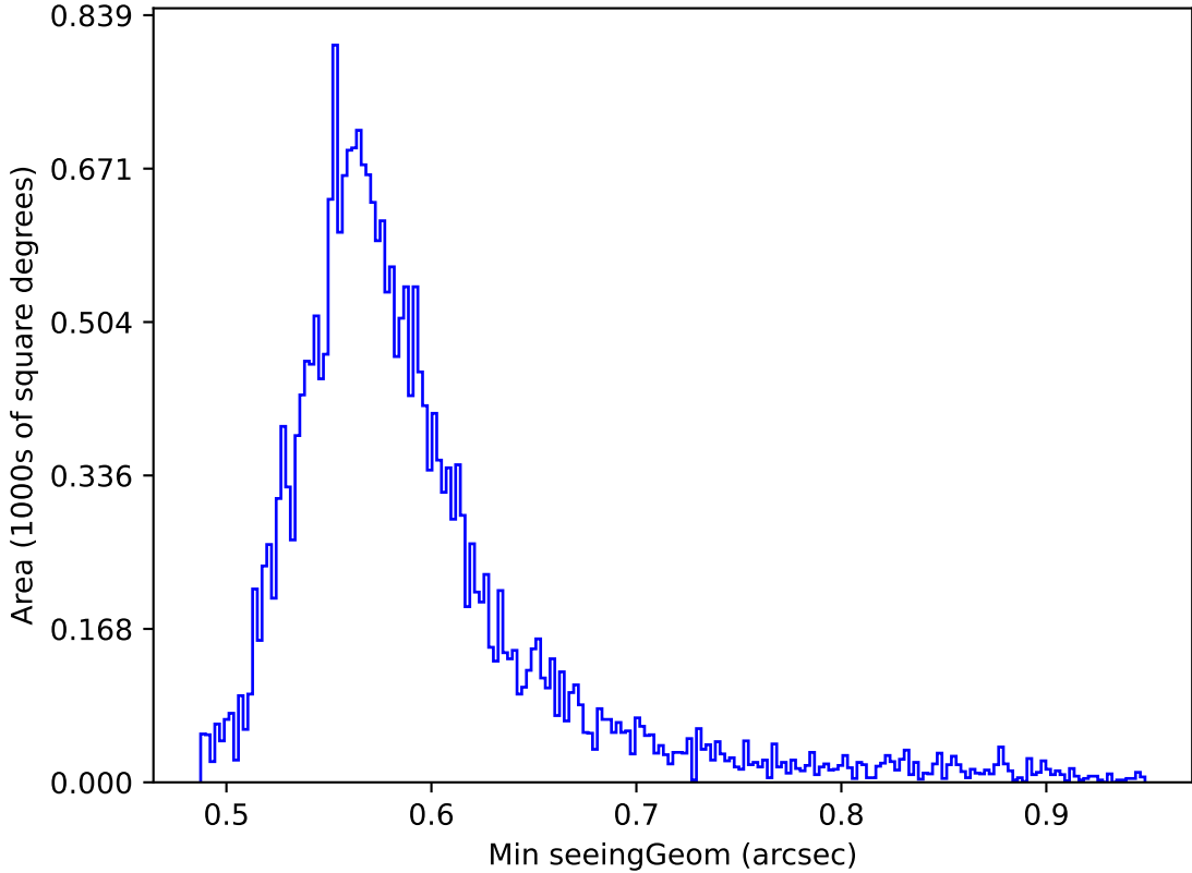
ddf_loaded_half_fl8_v3.4_10yrs Yr 1 all bands: Min seeingGeom
