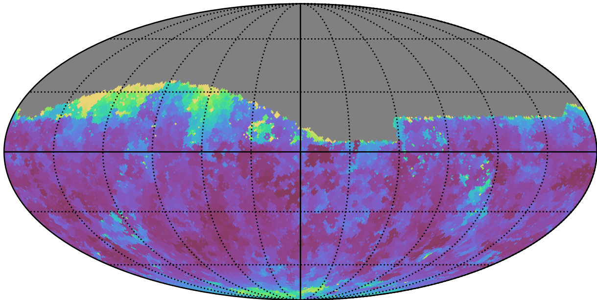
ddf_loaded_half_fl8_v3.4_10yrs Yr 1 z band: Min seeingEff
