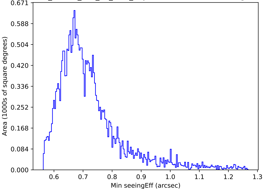
ddf_loaded_half_fl8_v3.4_10yrs Yr 1 z band: Min seeingEff
