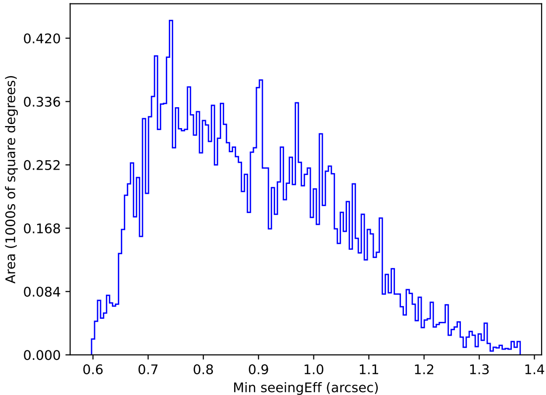
ddf_loaded_half_fl8_v3.4_10yrs Yr 1 u band: Min seeingEff
