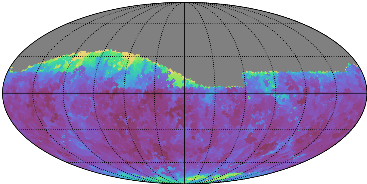
ddf_loaded_half_fl8_v3.4_10yrs Yr 1 i band: Min seeingEff
