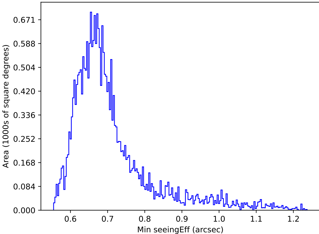
ddf_loaded_half_fl8_v3.4_10yrs Yr 1 i band: Min seeingEff
