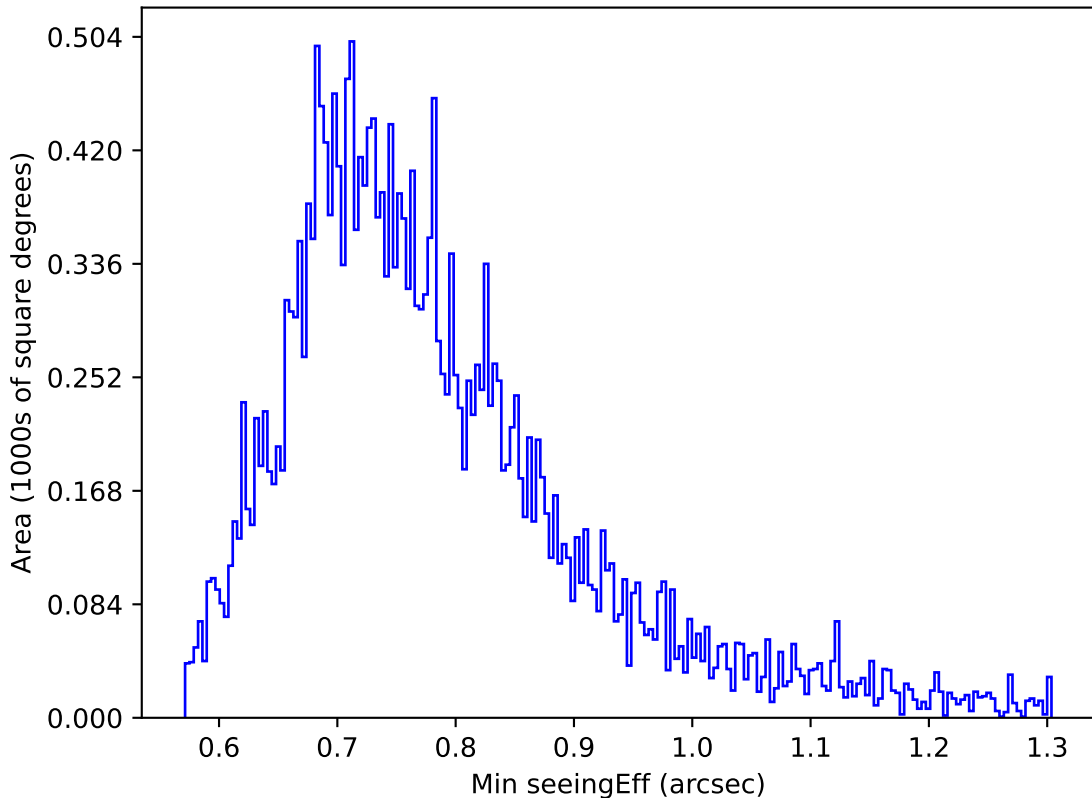
ddf_loaded_half_fl8_v3.4_10yrs Yr 1 g band: Min seeingEff
