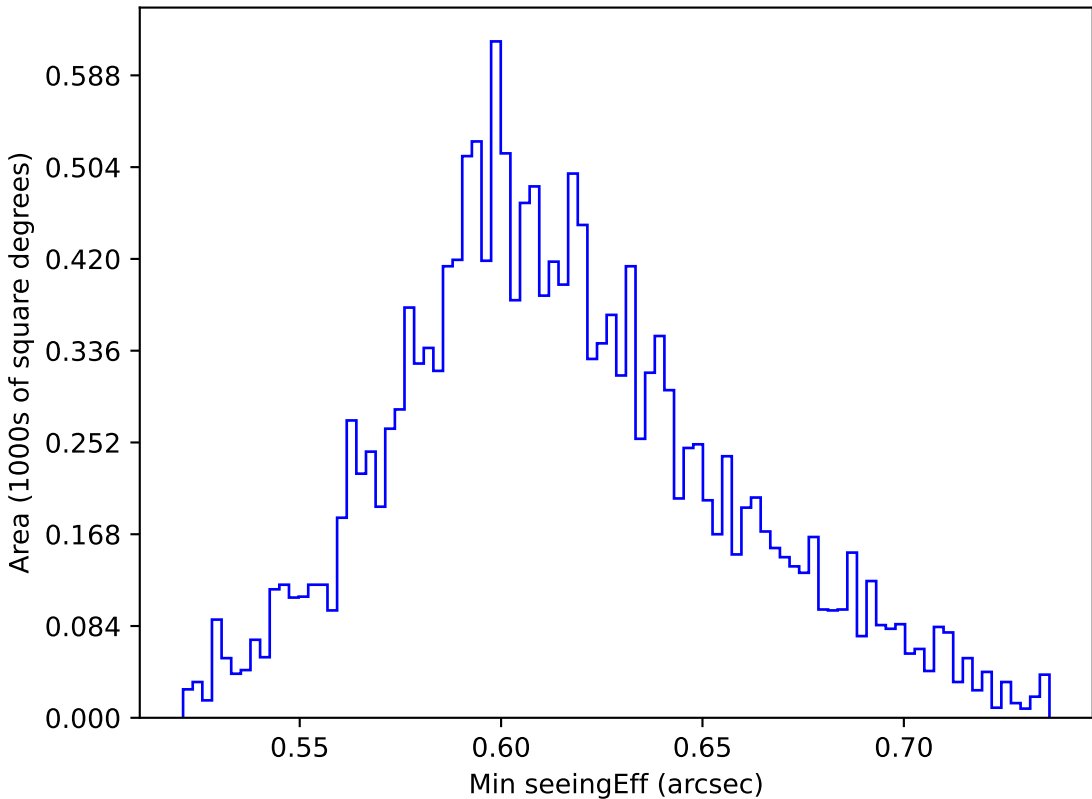
ddf_loaded_half_fl8_v3.4_10yrs WFD z band: Min seeingEff
