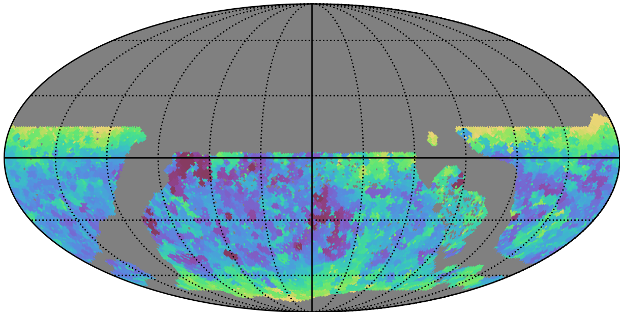
ddf_loaded_half_fl8_v3.4_10yrs WFD y band: Min seeingEff
