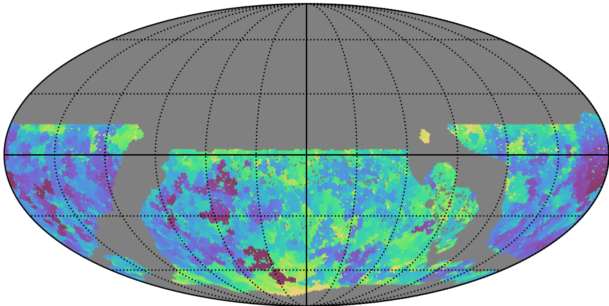
ddf_loaded_half_fl8_v3.4_10yrs WFD u band: Min seeingEff
