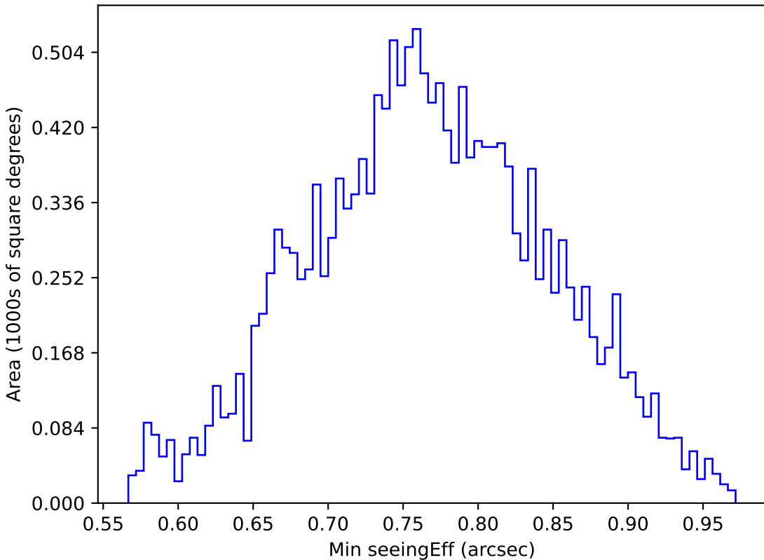
ddf_loaded_half_fl8_v3.4_10yrs WFD u band: Min seeingEff
