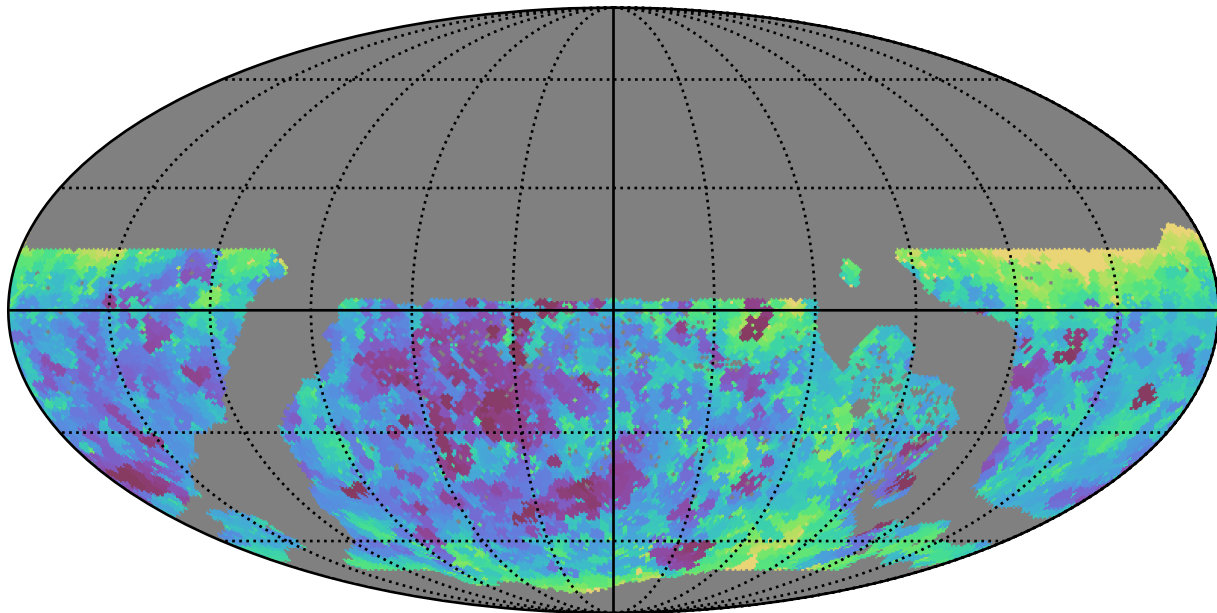
ddf_loaded_half_fl8_v3.4_10yrs WFD r band: Min seeingEff
