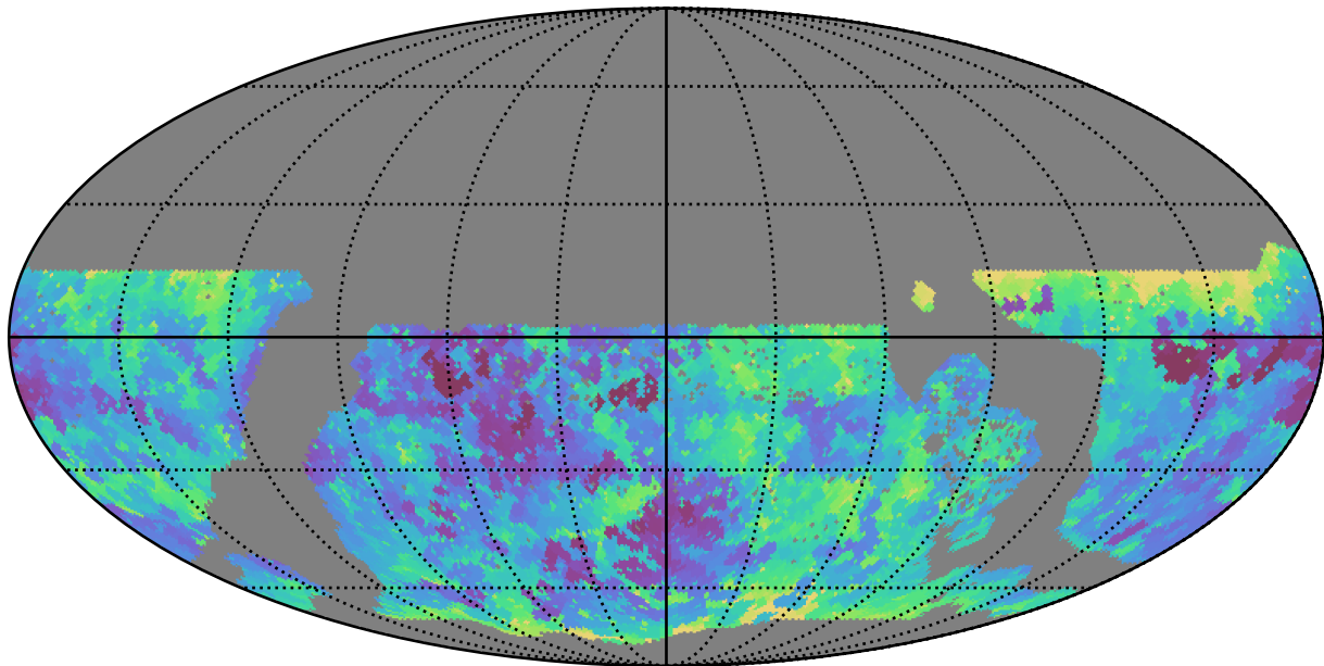
ddf_loaded_half_fl8_v3.4_10yrs WFD g band: Min seeingEff
