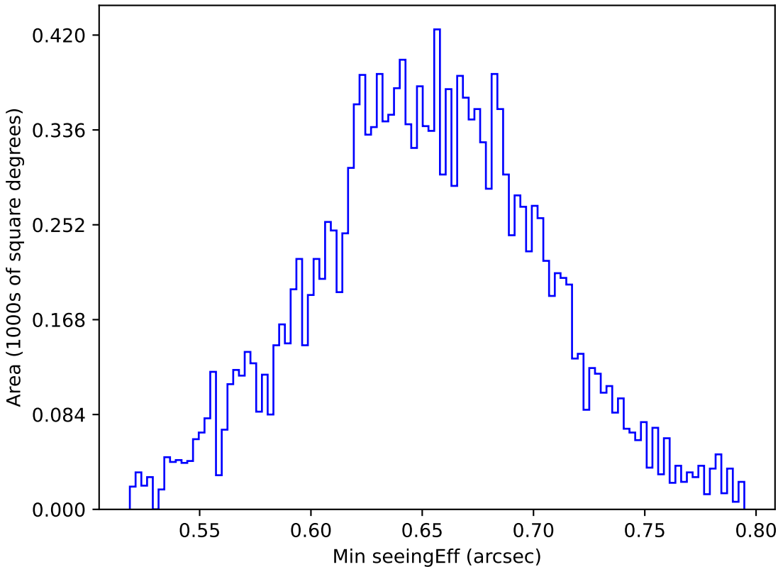
ddf_loaded_half_fl8_v3.4_10yrs WFD g band: Min seeingEff
