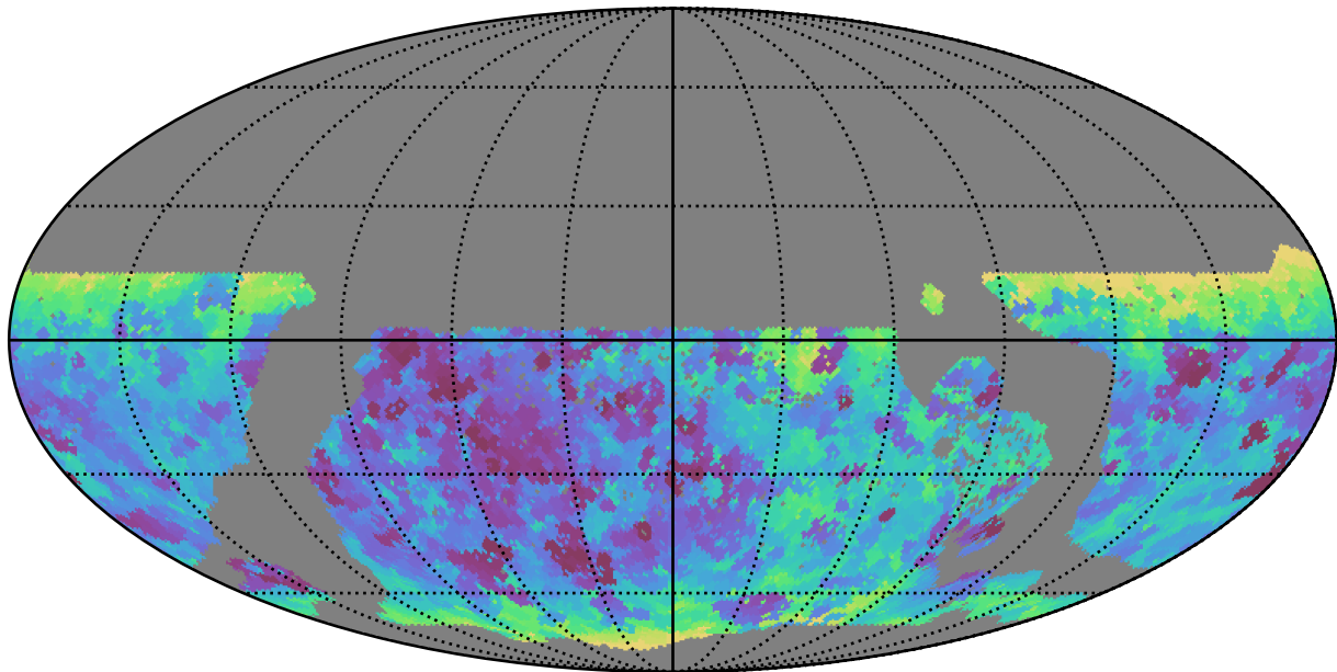
ddf_loaded_half_fl8_v3.4_10yrs WFD all bands: Min seeingEff
