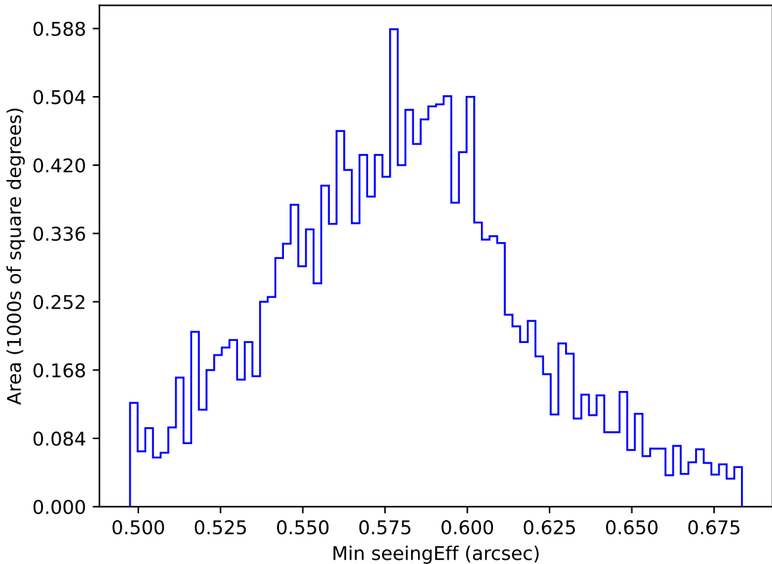
ddf_loaded_half_fl8_v3.4_10yrs WFD all bands: Min seeingEff
