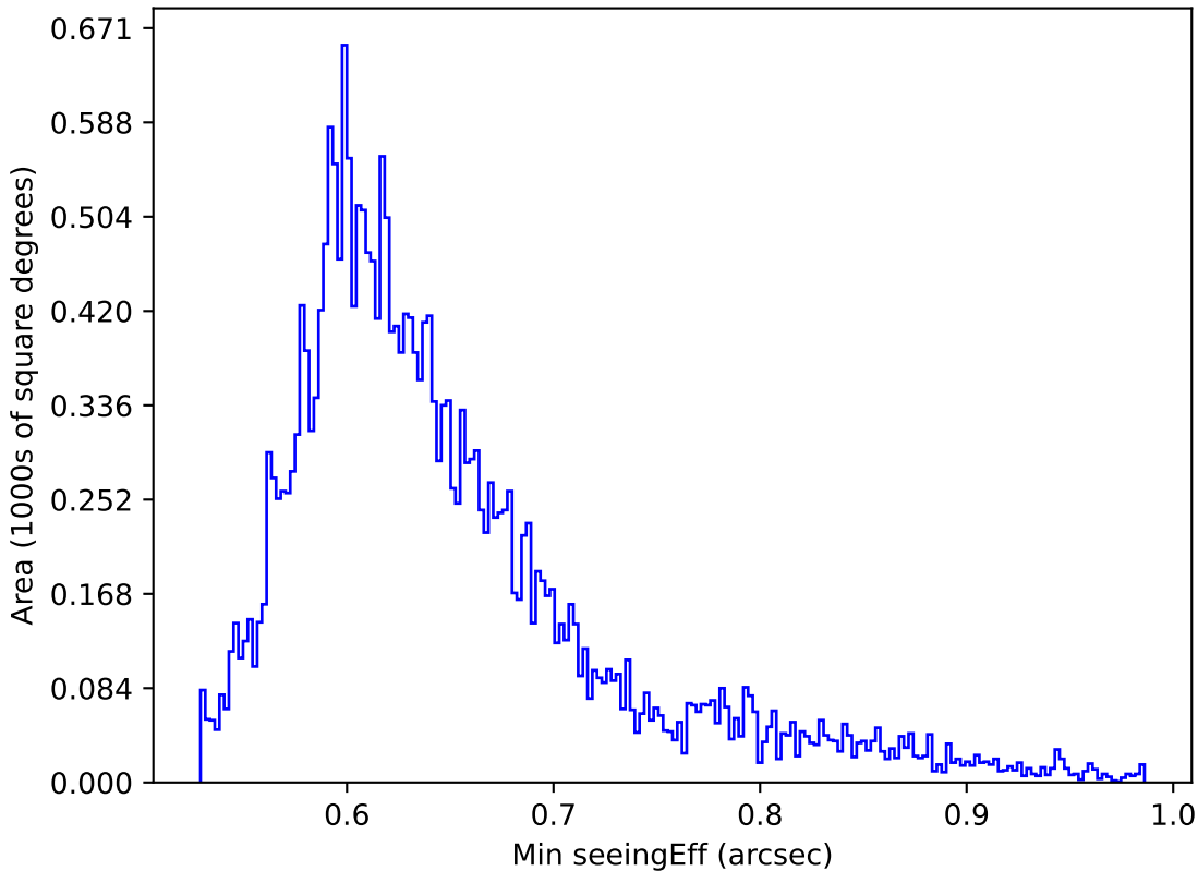
ddf_loaded_half_fl8_v3.4_10yrs All sky z band: Min seeingEff
