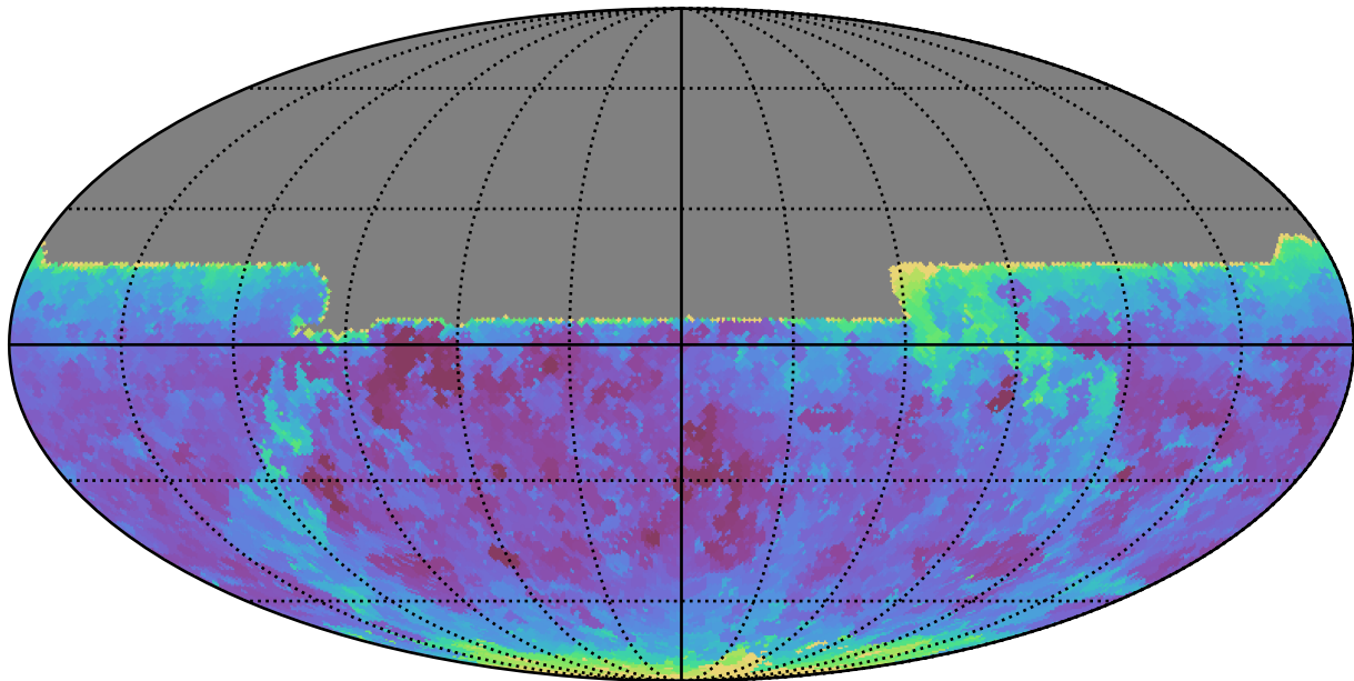
ddf_loaded_half_fl8_v3.4_10yrs All sky y band: Min seeingEff
