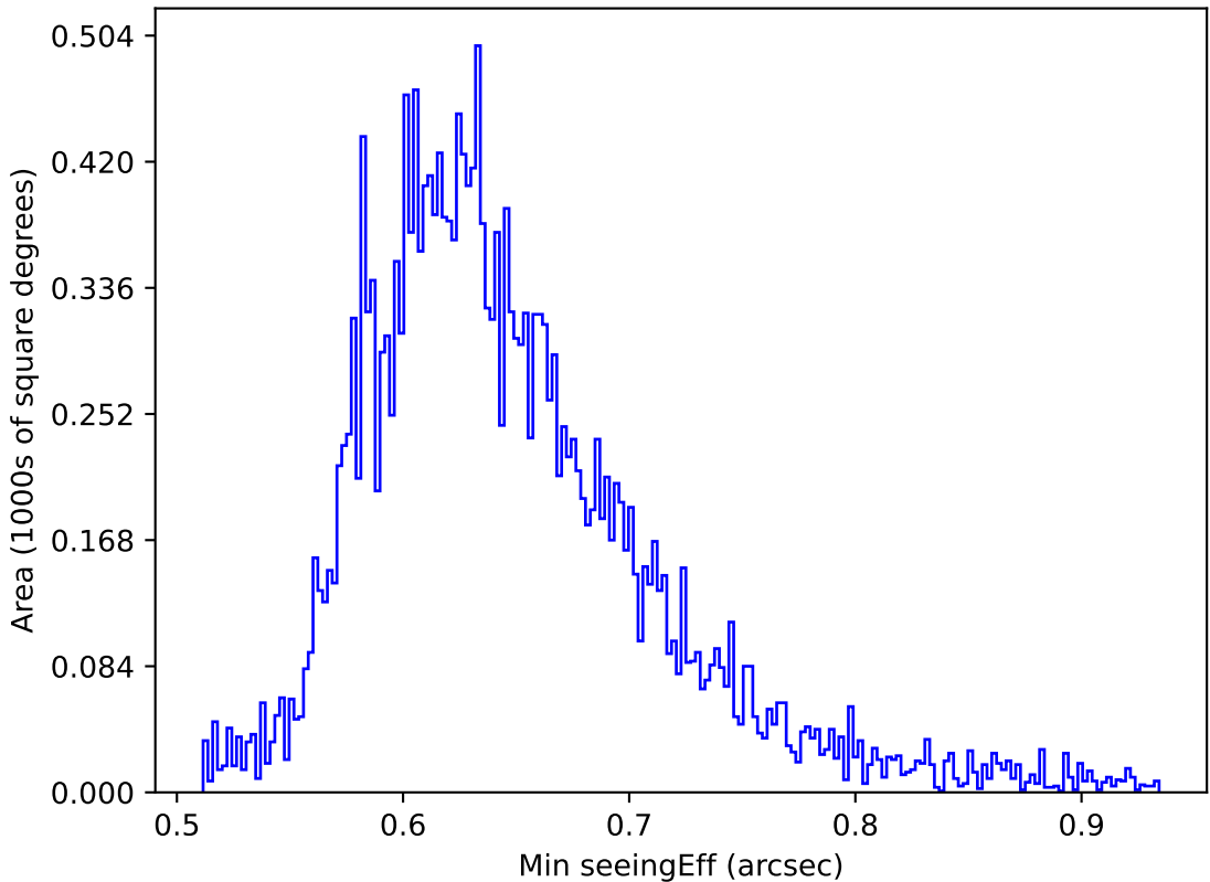
ddf_loaded_half_fl8_v3.4_10yrs All sky y band: Min seeingEff
