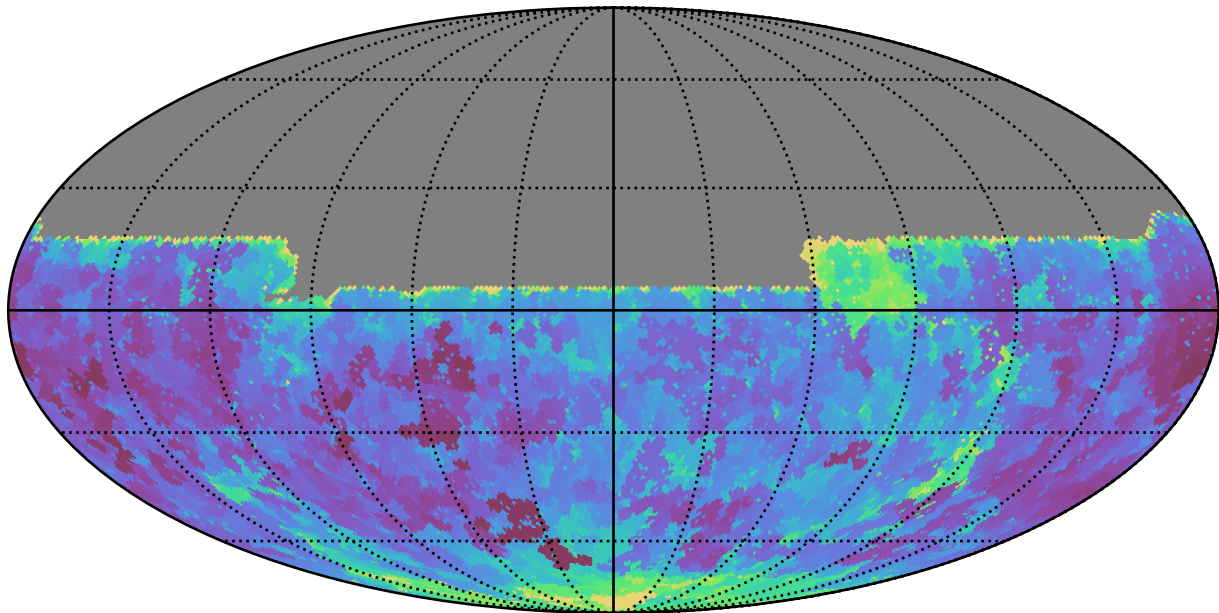
ddf_loaded_half_fl8_v3.4_10yrs All sky u band: Min seeingEff
