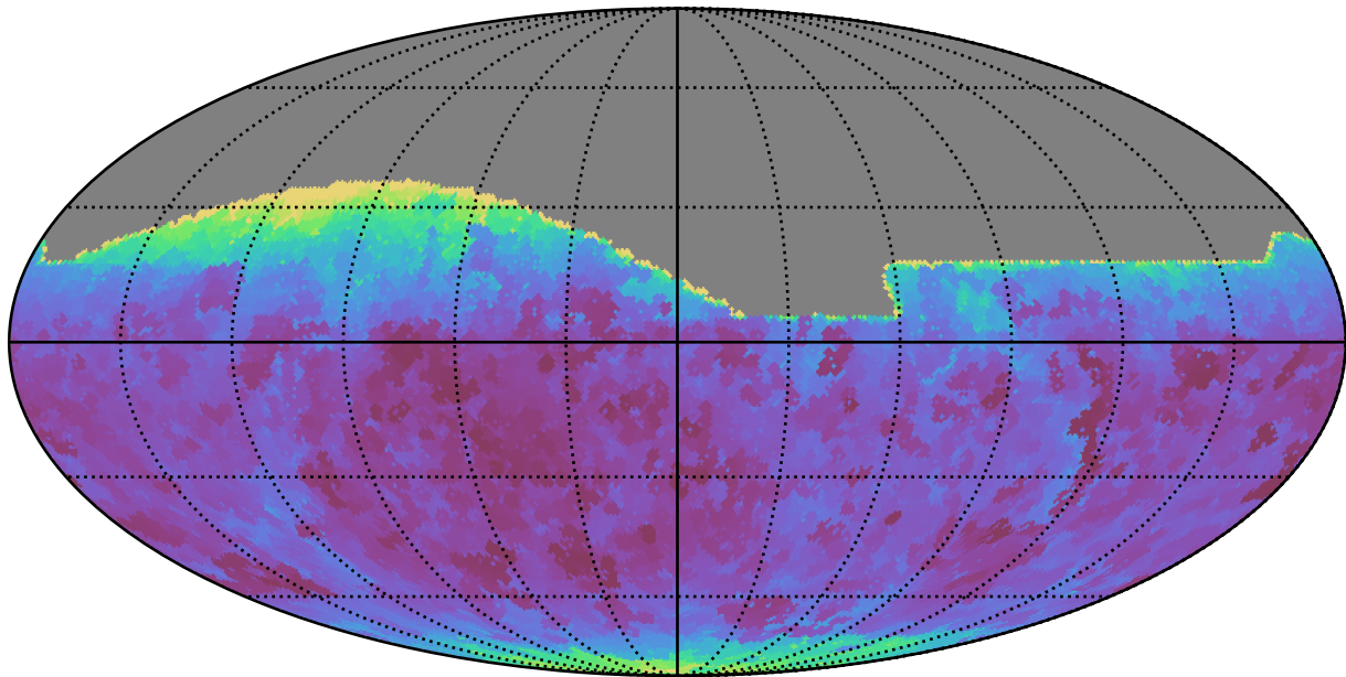
ddf_loaded_half_fl8_v3.4_10yrs All sky all bands: Min seeingEff
