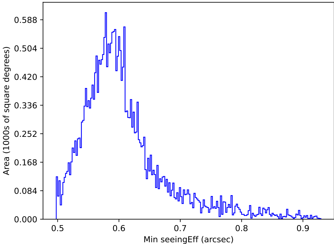
ddf_loaded_half_fl8_v3.4_10yrs All sky all bands: Min seeingEff
