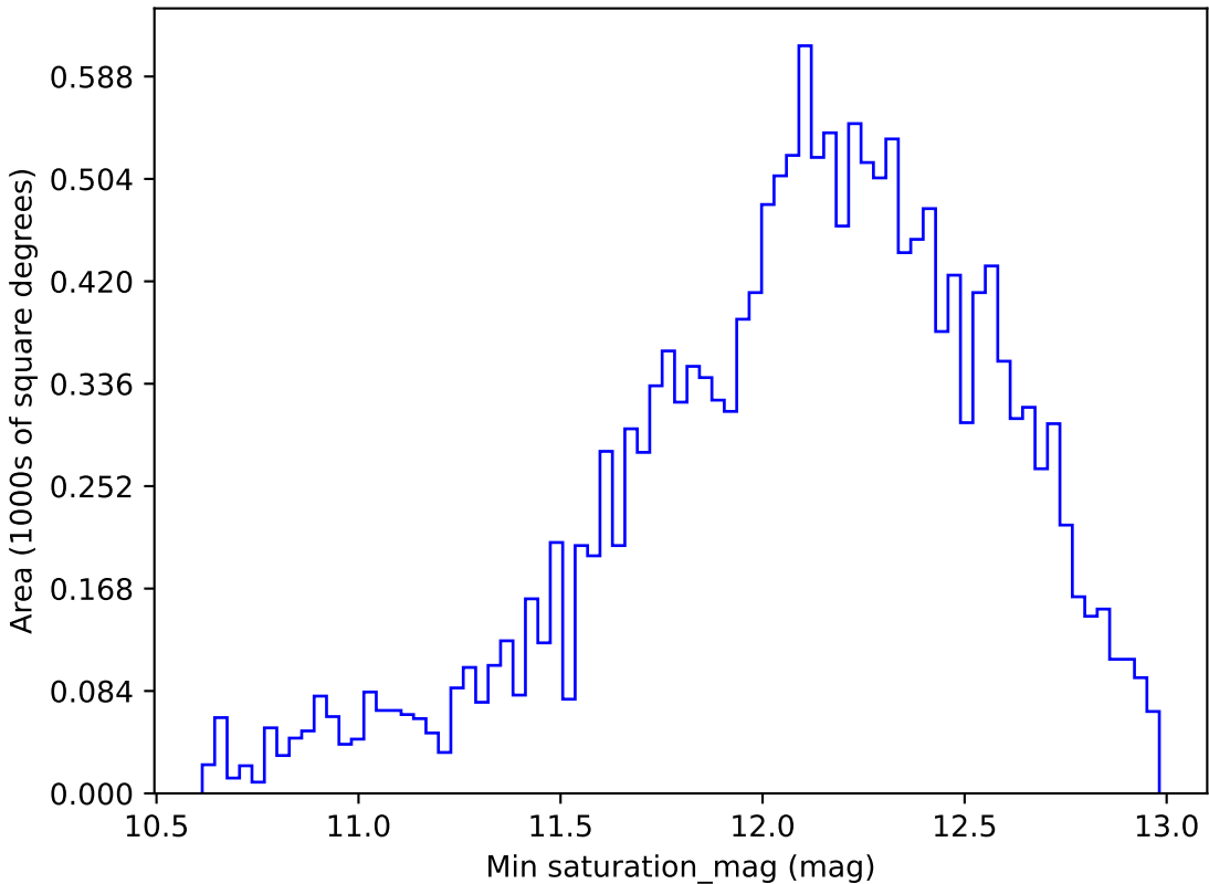
ddf_loaded_half_fl8_v3.4_10yrs WFD z band: Min saturation_mag
