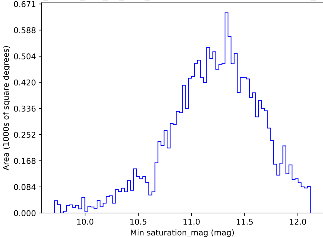
ddf_loaded_half_fl8_v3.4_10yrs WFD y band: Min saturation_mag
