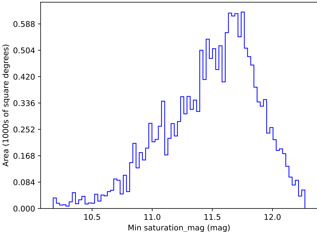
ddf_loaded_half_fl8_v3.4_10yrs WFD u band: Min saturation_mag
