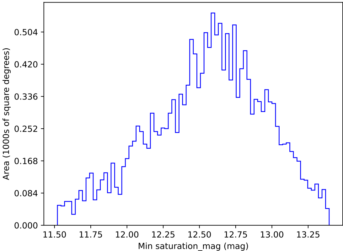
ddf_loaded_half_fl8_v3.4_10yrs WFD r band: Min saturation_mag
