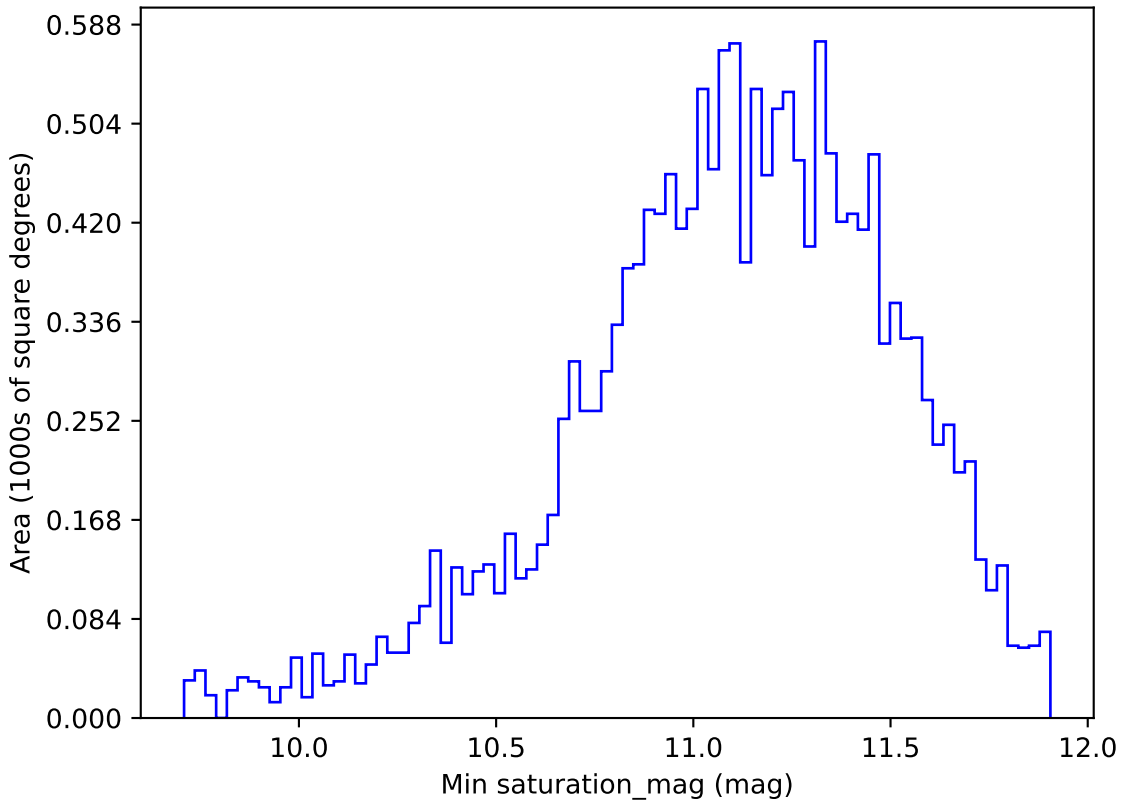
ddf_loaded_half_fl8_v3.4_10yrs WFD all bands: Min saturation_mag
