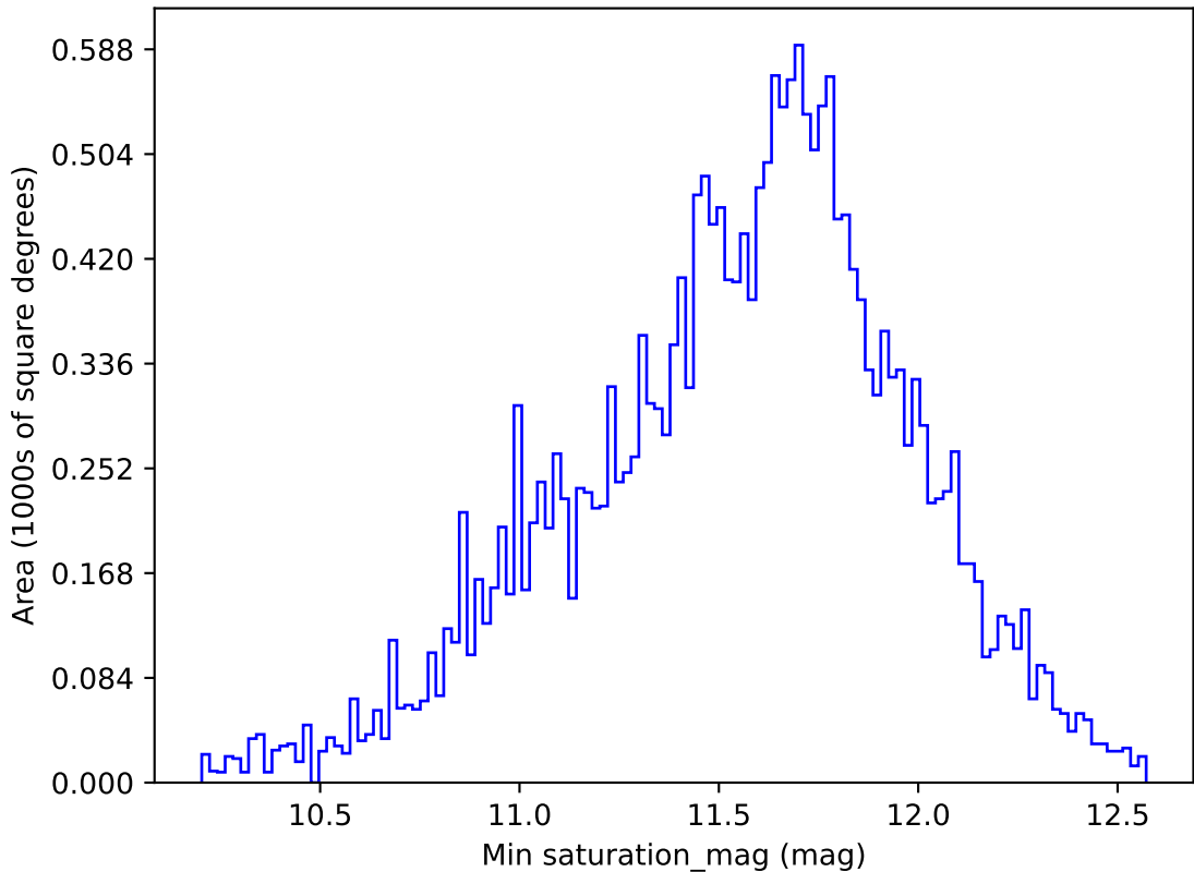
ddf_loaded_half_fl8_v3.4_10yrs All sky u band: Min saturation_mag
