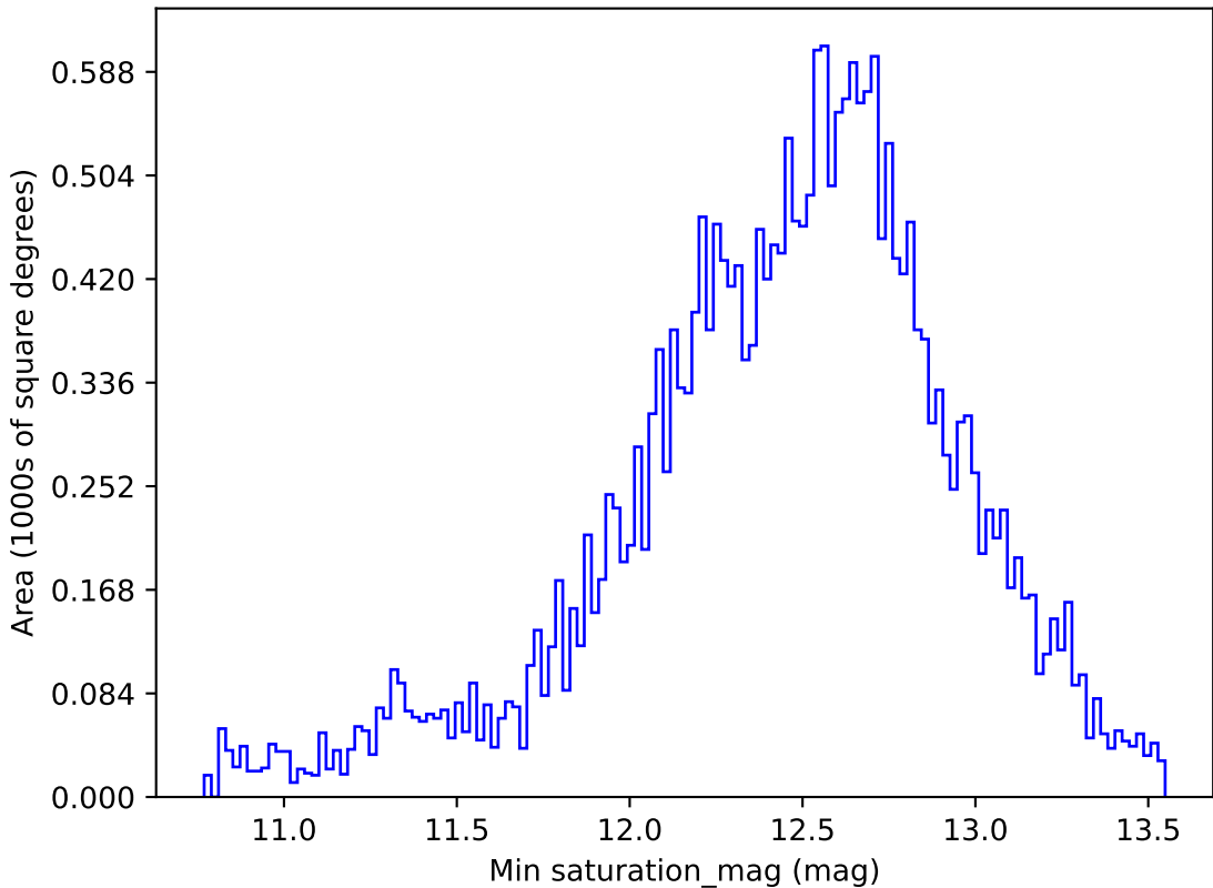
ddf_loaded_half_fl8_v3.4_10yrs All sky i band: Min saturation_mag
