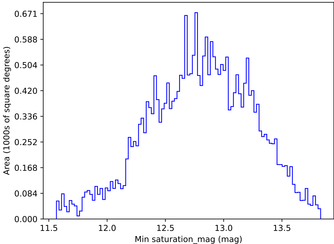
ddf_loaded_half_fl8_v3.4_10yrs All sky g band: Min saturation_mag
