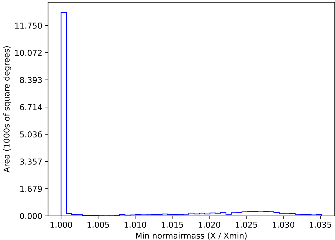
ddf_loaded_half_fl8_v3.4_10yrs WFD z band: Min normairmass
