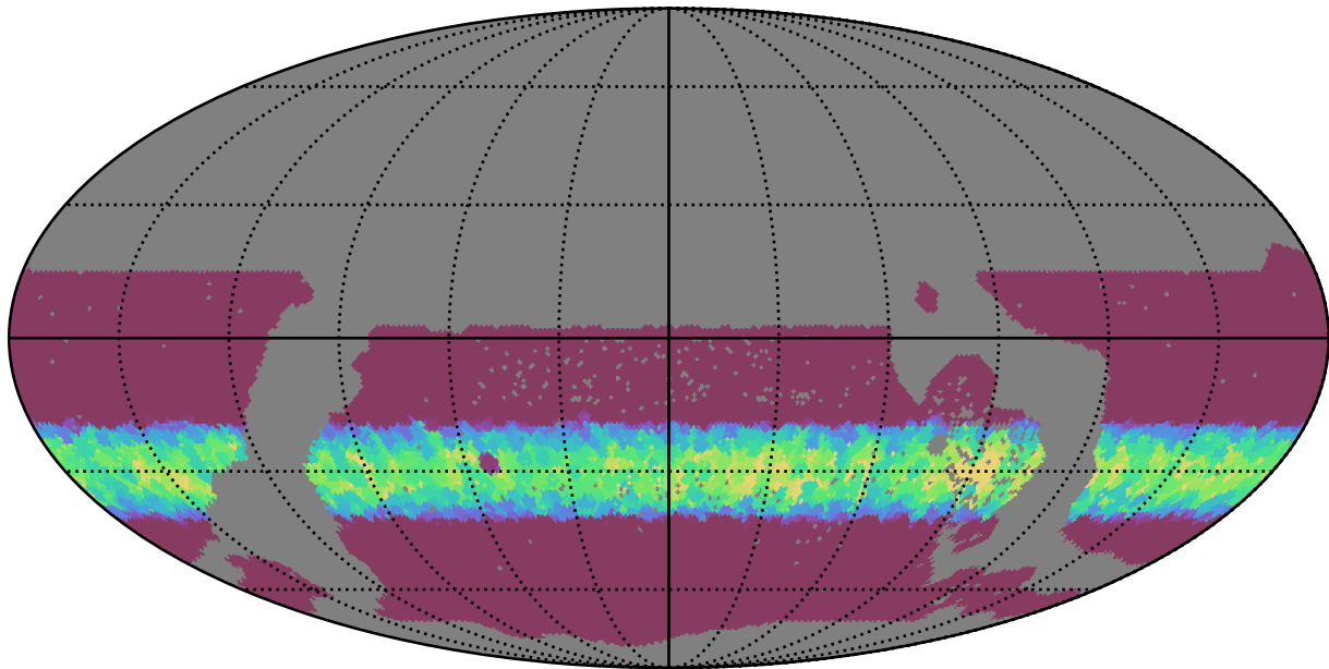
ddf_loaded_half_fl8_v3.4_10yrs WFD y band: Min normairmass
