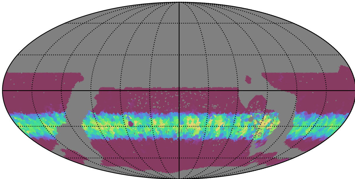
ddf_loaded_half_fl8_v3.4_10yrs WFD u band: Min normairmass
