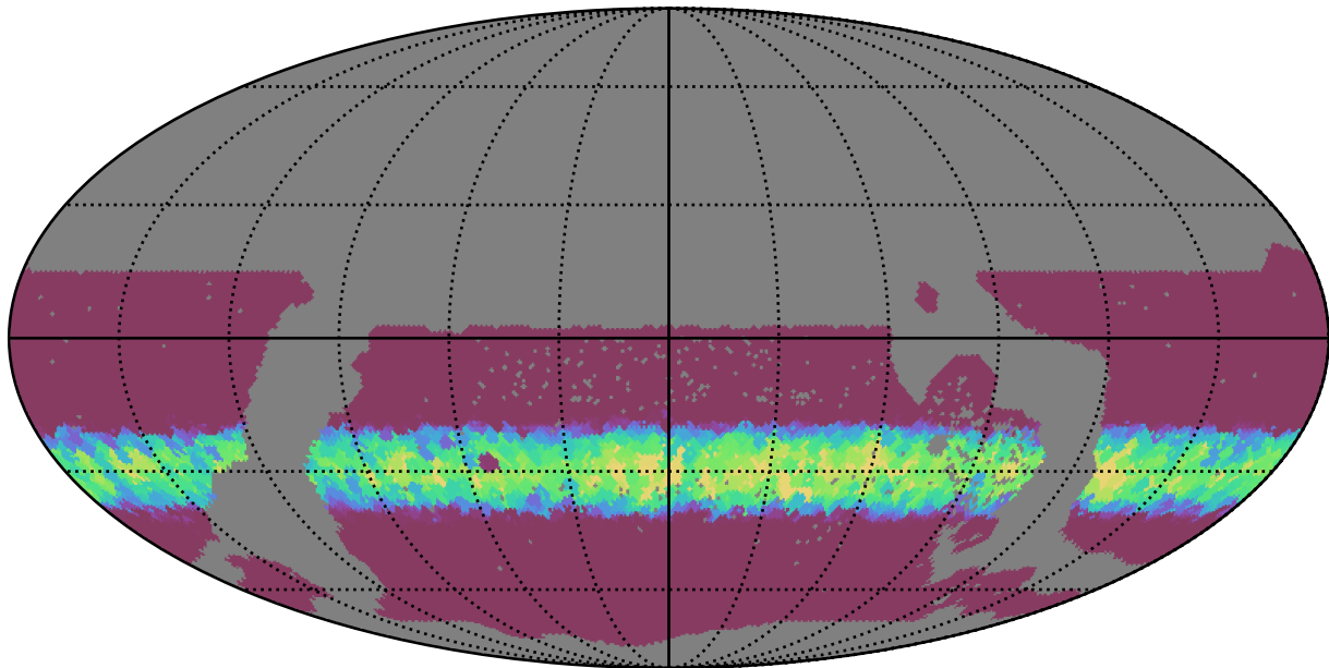
ddf_loaded_half_fl8_v3.4_10yrs WFD r band: Min normairmass
