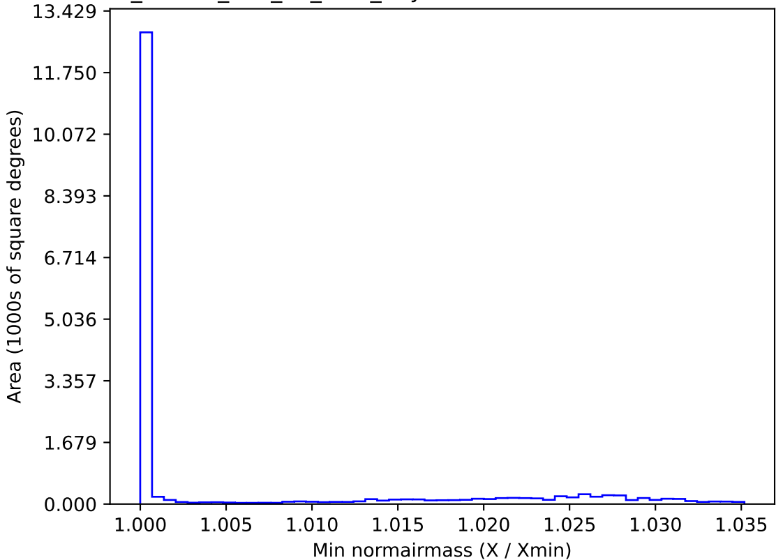
ddf_loaded_half_fl8_v3.4_10yrs WFD r band: Min normairmass
