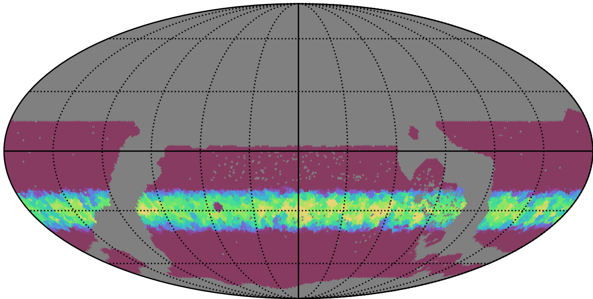
ddf_loaded_half_fl8_v3.4_10yrs WFD i band: Min normairmass
