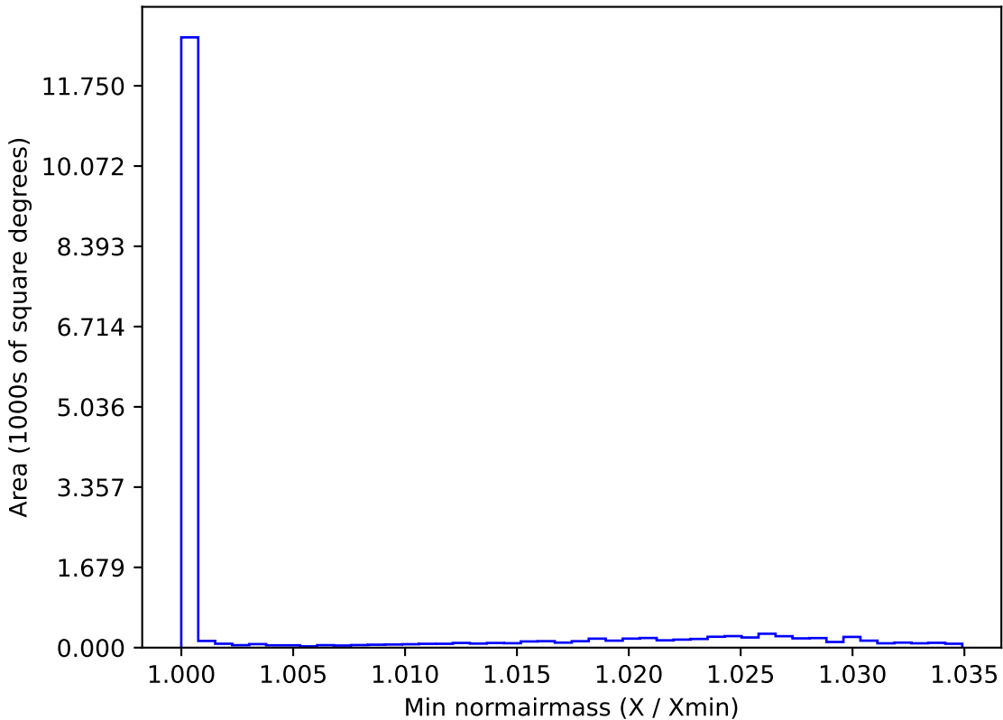
ddf_loaded_half_fl8_v3.4_10yrs WFD i band: Min normairmass
