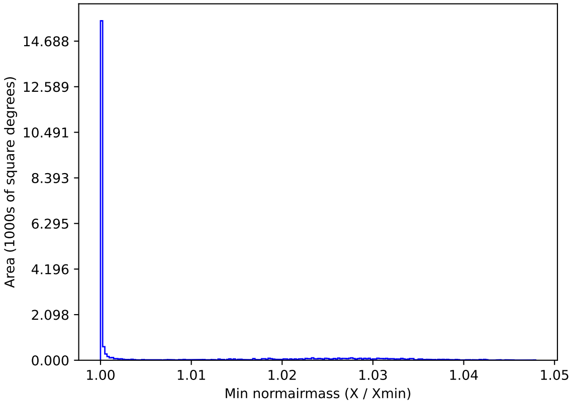
ddf_loaded_half_fl8_v3.4_10yrs All sky y band: Min normairmass
