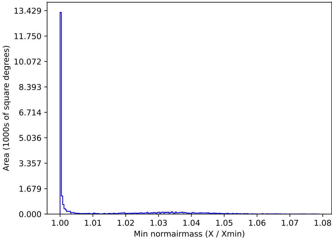
ddf_loaded_half_fl8_v3.4_10yrs All sky u band: Min normairmass
