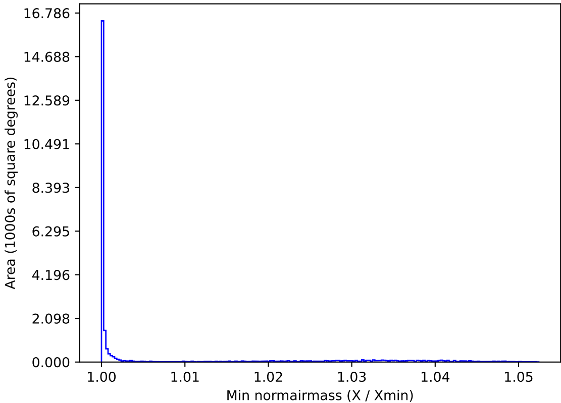
ddf_loaded_half_fl8_v3.4_10yrs All sky g band: Min normairmass
