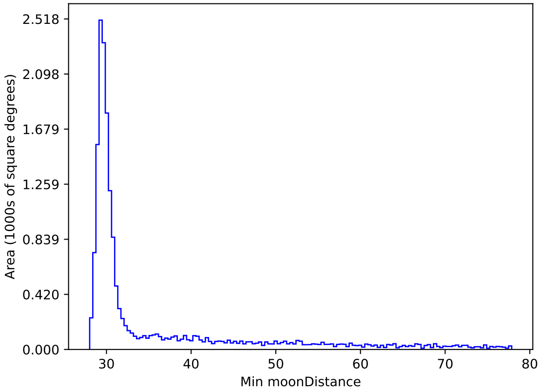
ddf_loaded_half_fl8_v3.4_10yrs WFD z band: Min moonDistance
