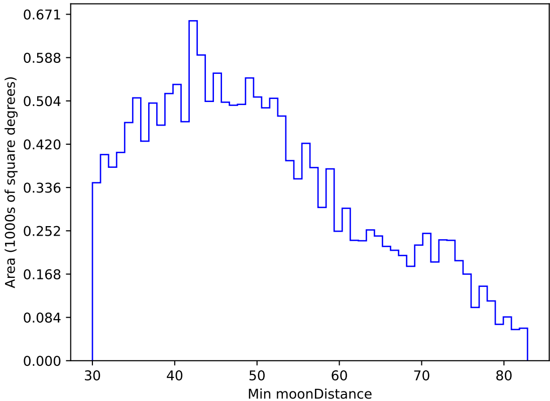
ddf_loaded_half_fl8_v3.4_10yrs WFD u band: Min moonDistance
