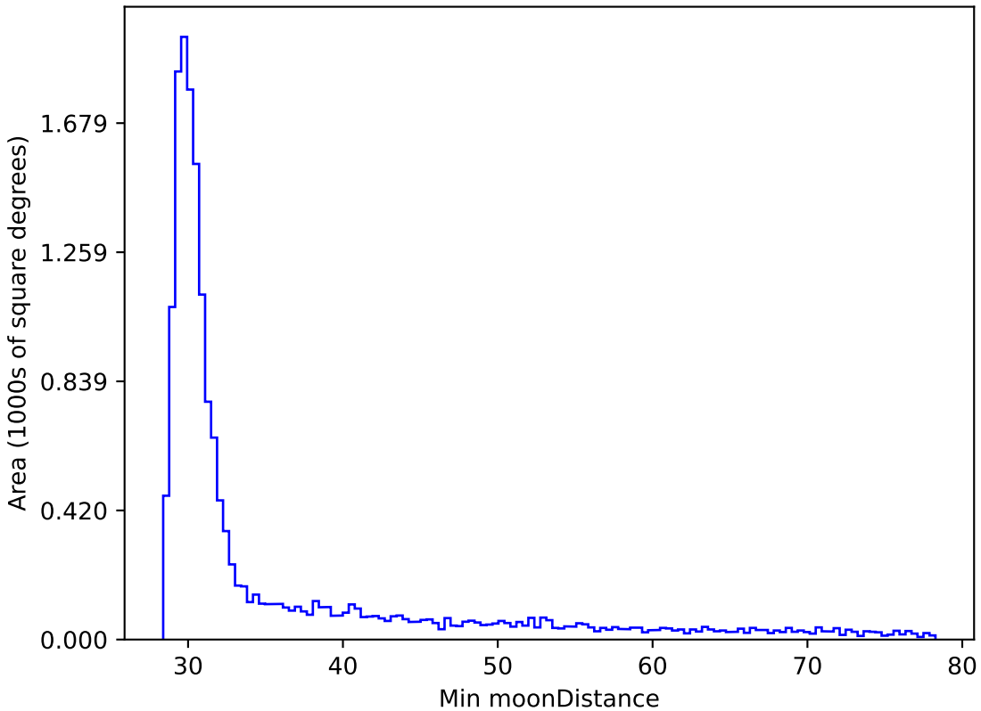
ddf_loaded_half_fl8_v3.4_10yrs WFD i band: Min moonDistance
