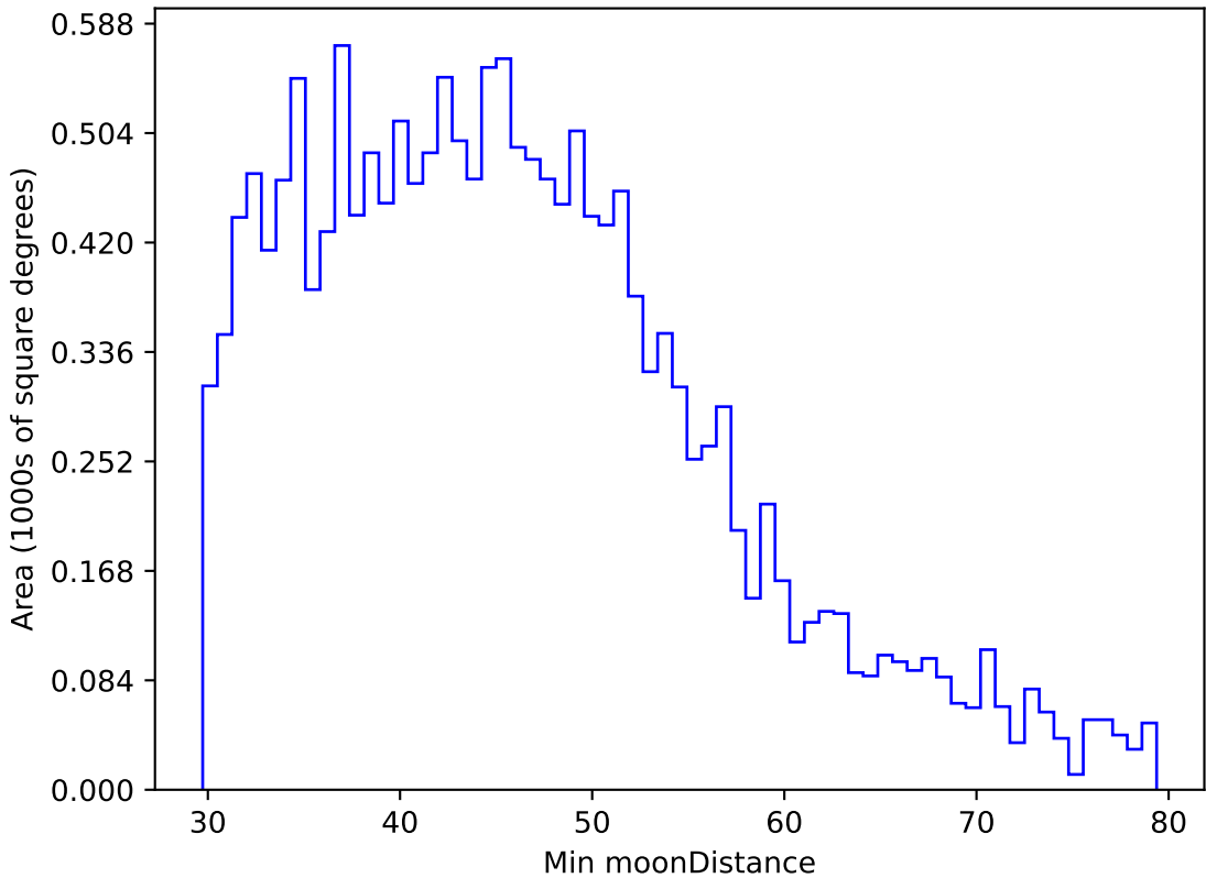
ddf_loaded_half_fl8_v3.4_10yrs WFD g band: Min moonDistance
