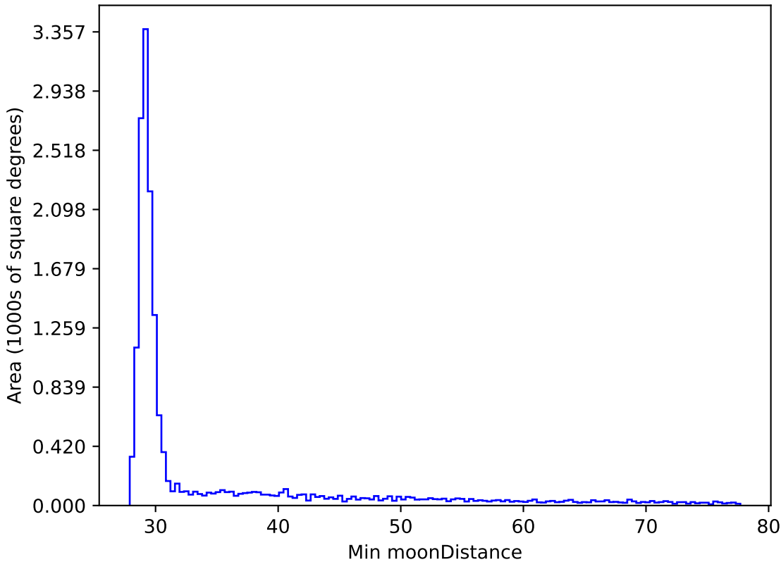
ddf_loaded_half_fl8_v3.4_10yrs WFD all bands: Min moonDistance
