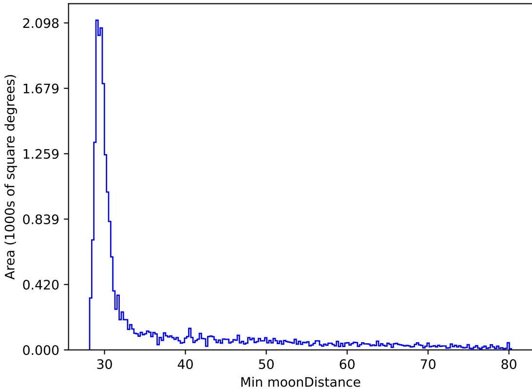
ddf_loaded_half_fl8_v3.4_10yrs All sky y band: Min moonDistance
