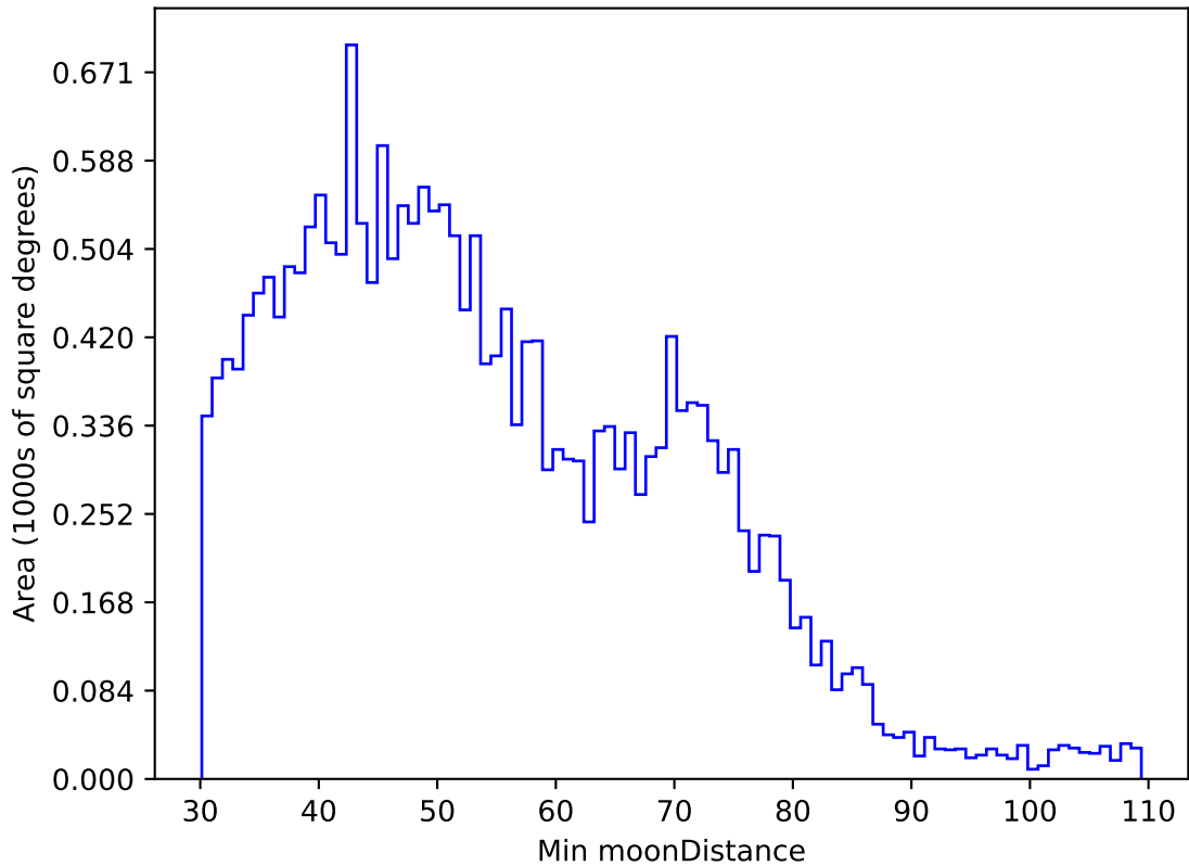
ddf_loaded_half_fl8_v3.4_10yrs All sky u band: Min moonDistance
